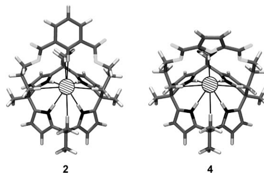
Figure 4. Optimized B3LYP/DZVP2 geometries of the chloride anion complex of the benzene-strapped calix[4]pyrrole 2 and the furan-strapped calix[4]pyrrole 4 . A corresponding view for the pyrrole-strapped system 3 , as well as Cartesian coordinates and absolute energies for all three species, is included in the Supporting Information.
